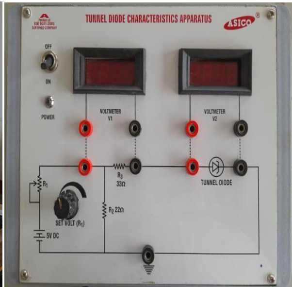
Tunnel Diode Characteristics Apparatus
