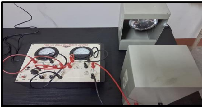
Photo Cell Characteristics apparatus
