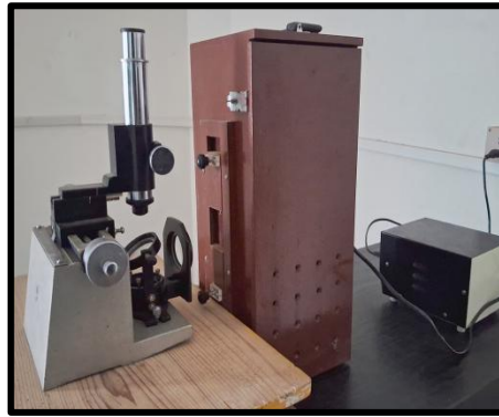
Newton ring experiment setup
