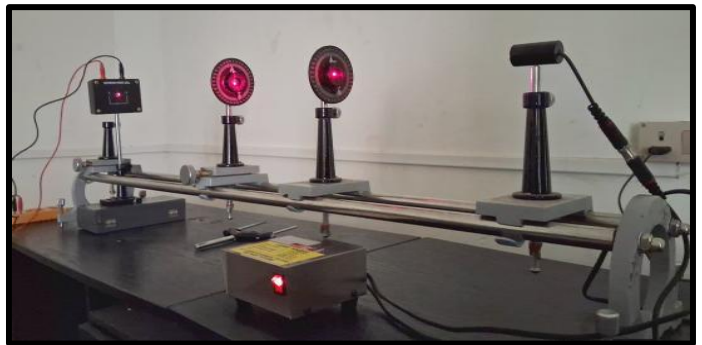
Set for verification for Malus's law
